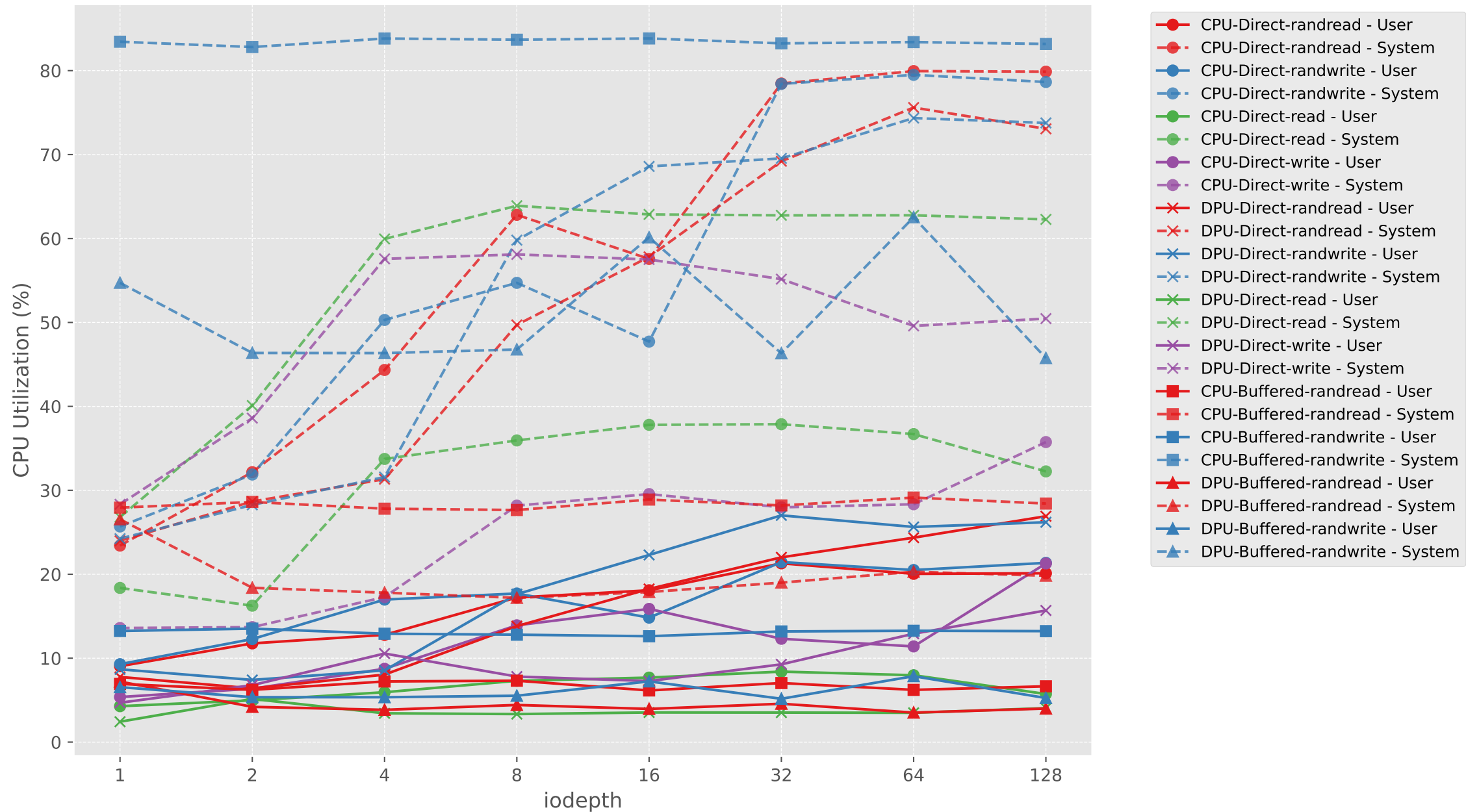
CPU Utilization vs iodepth (CPU vs DPU, Direct vs Buffered)
